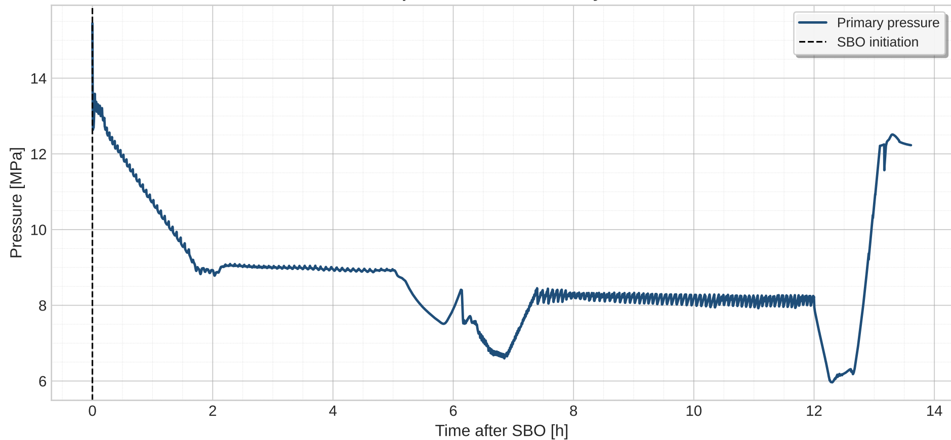
No SG Depressurization - Primary Pressure
